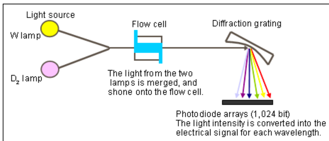
Figure2. Diagrammatic illustration of a DAD optical system
